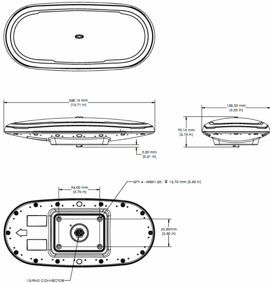
Figure 2-5: V200s dimensions
