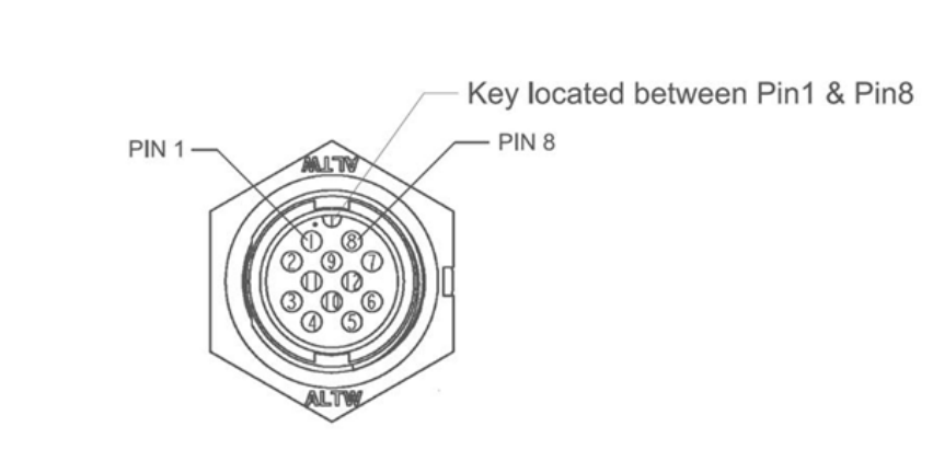
Figure 3-1: V200s pin-out assignments
