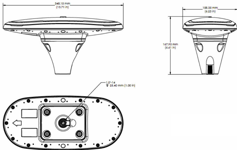
Figure 2-6: V200s with pole mount accessory
