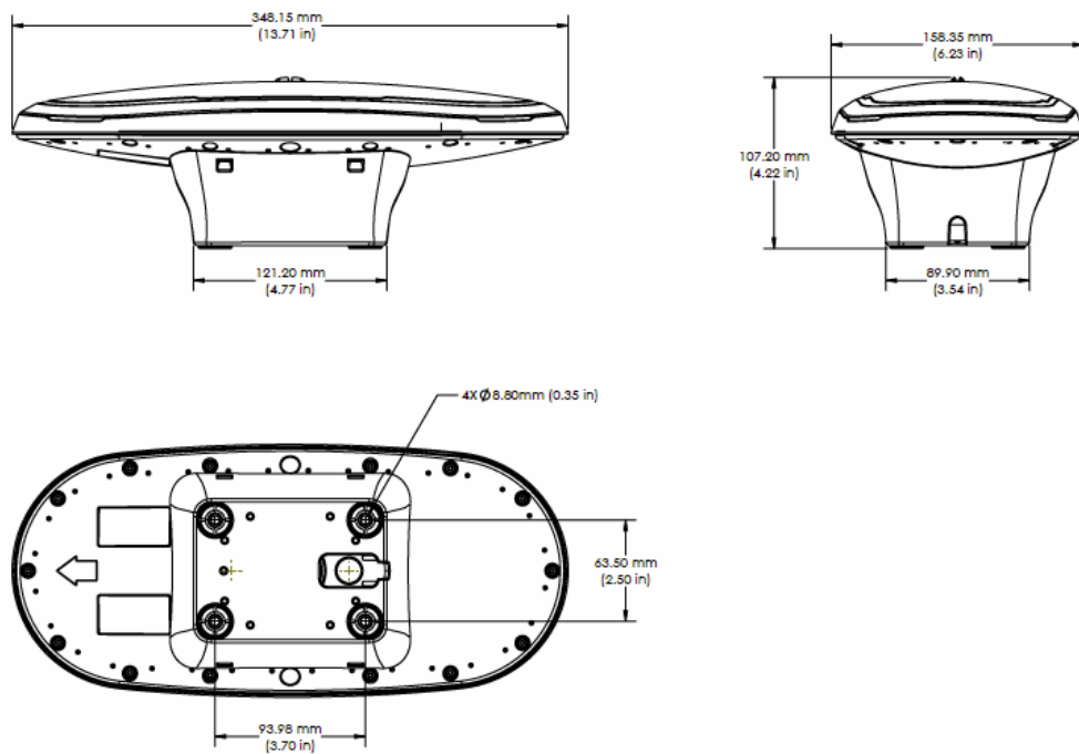
Figure 2-8: V200s with high-profile mount accessory
