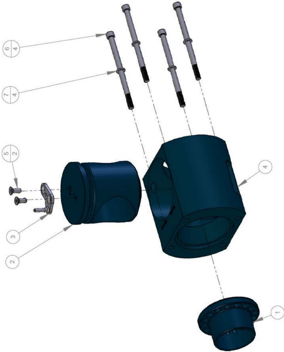
Figure B.4. Merlin Diffuser Assembly
