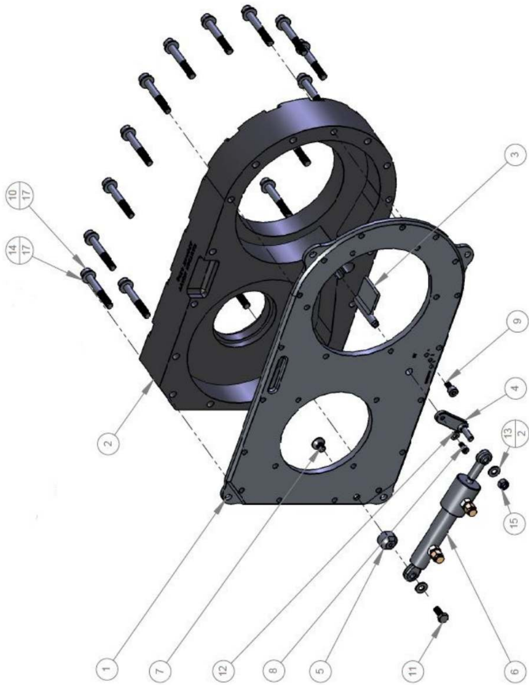
Figure B.2. Merlin Body
