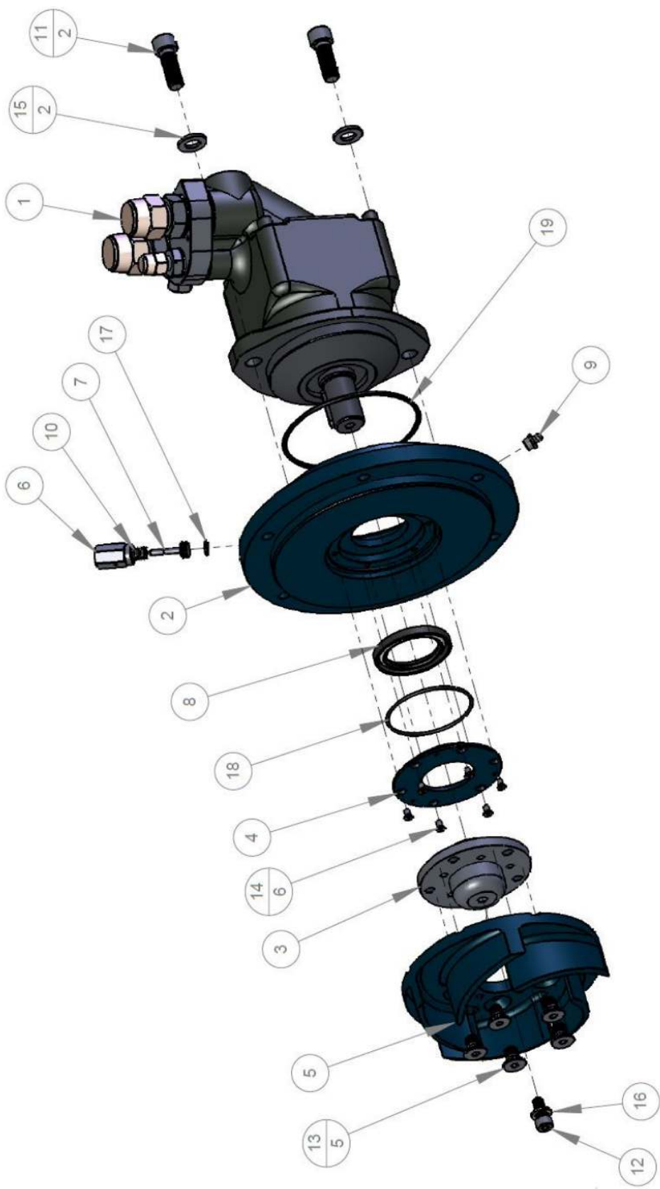
Figure B.3. Merlin Motor Mount Assembly
