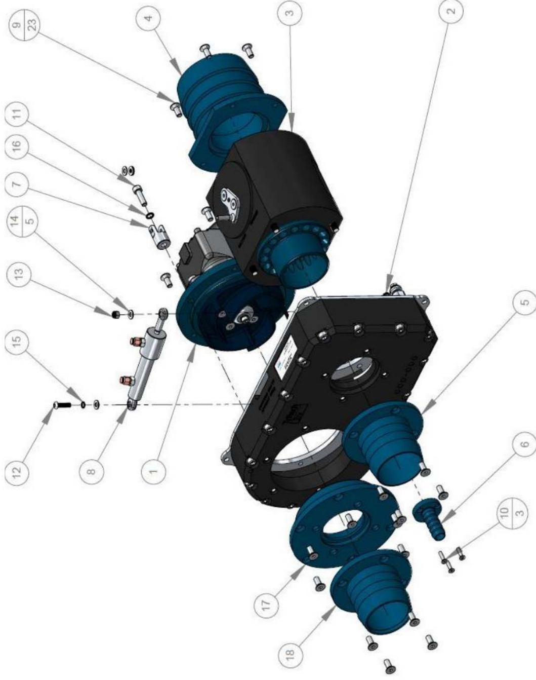
Figure B.1. Main Pump
